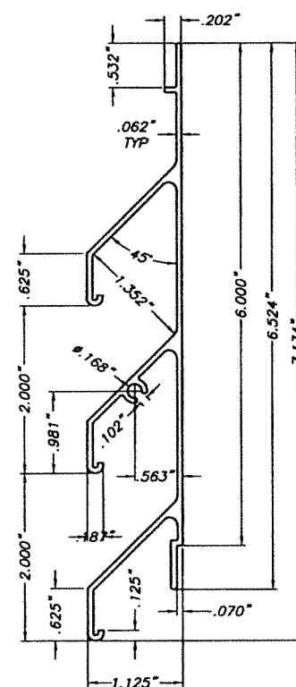
J SHUTTER BLADE SCALE: 1/2" = 1"
