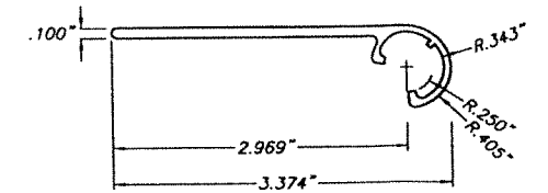
D FLAT FEMALE HINGE SCALE: 1/2" = 1"
