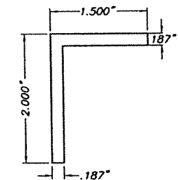
N WALL MOUNT Alum. BRACKET 7" LONG SCALE: 1/2" = 1"
